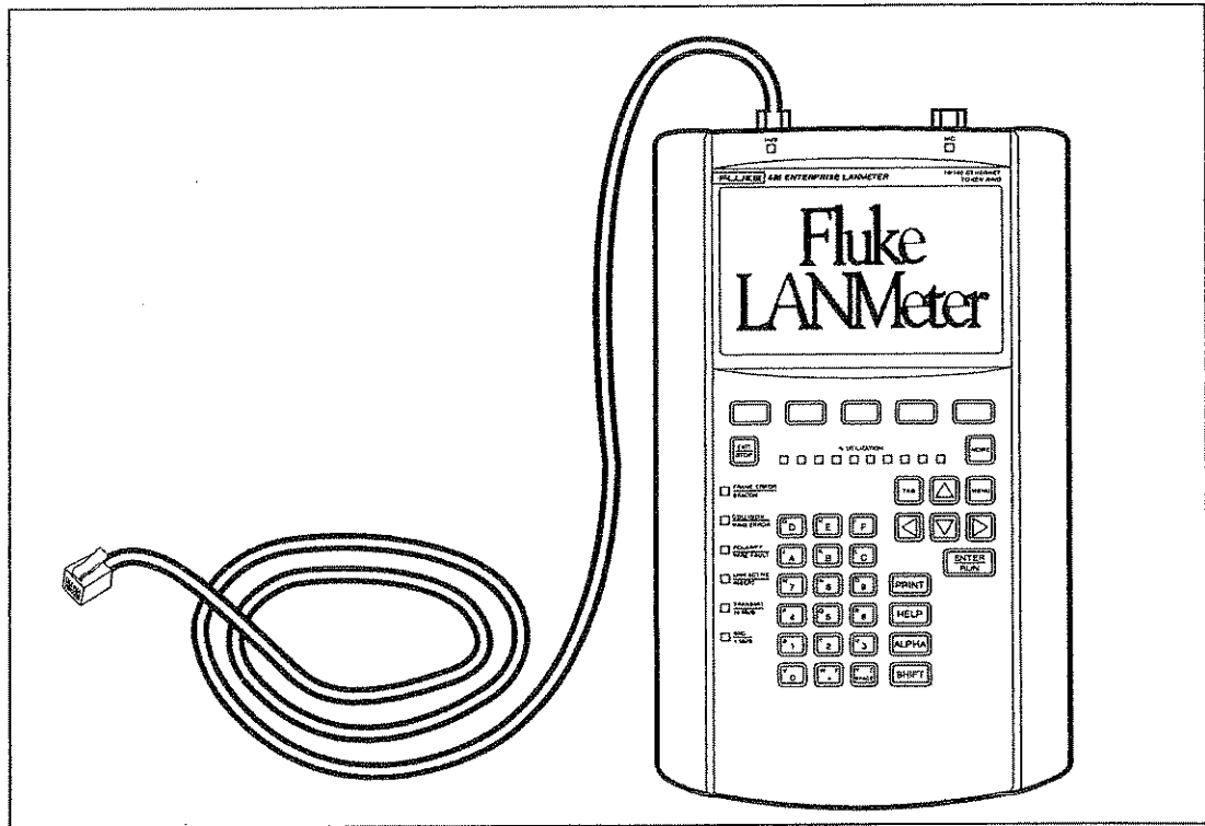
Figure A-5. Bad Cable Test Connection
